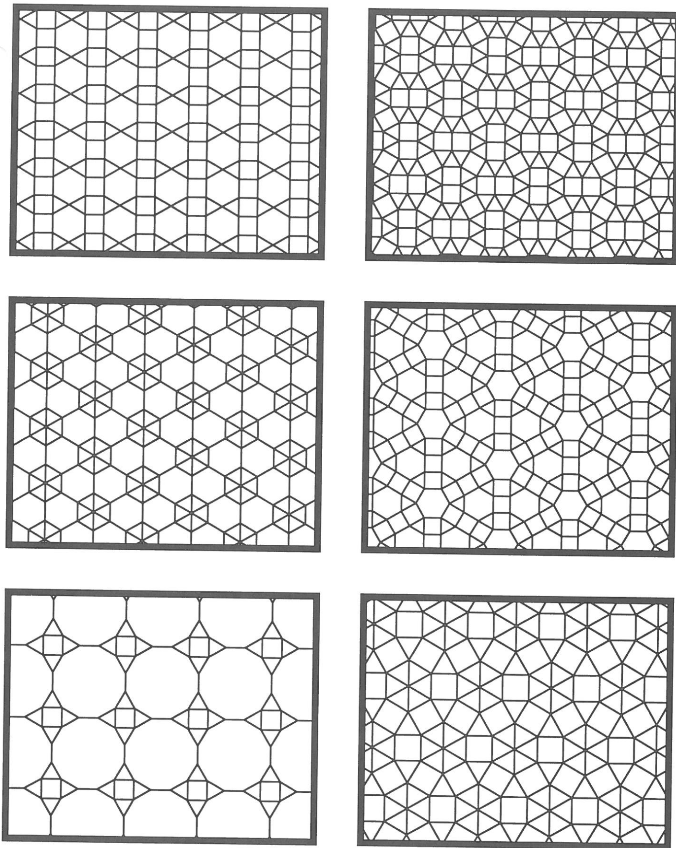
Fig. 3-24. Tessellations of regular polygons that contain more than one type of vertex point
