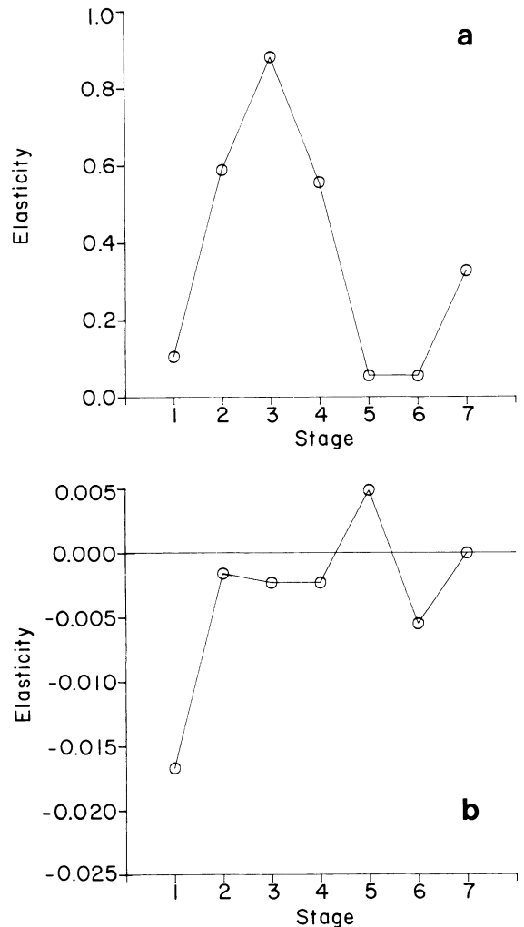
FIG. 4. (a) The elasticity, or proportional sensitivity, of \lambda_m to changes in annual stage-specific survival probability p_i . (b) The elasticity of \lambda_m to changes in stage duration d_i . Elasticity in stage duration is negative because stage duration and population growth rates r are inversely related. Overall, proportional sensitivity is much higher to survival than to stage duration.
