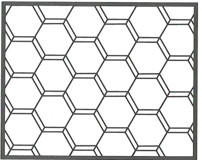
Fig. 5-22. Hexagonal grid and five tessellations of overlapping hexagons
